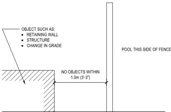
FENCE SECTION
