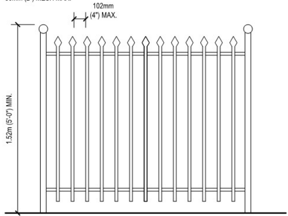
METAL FENCE
